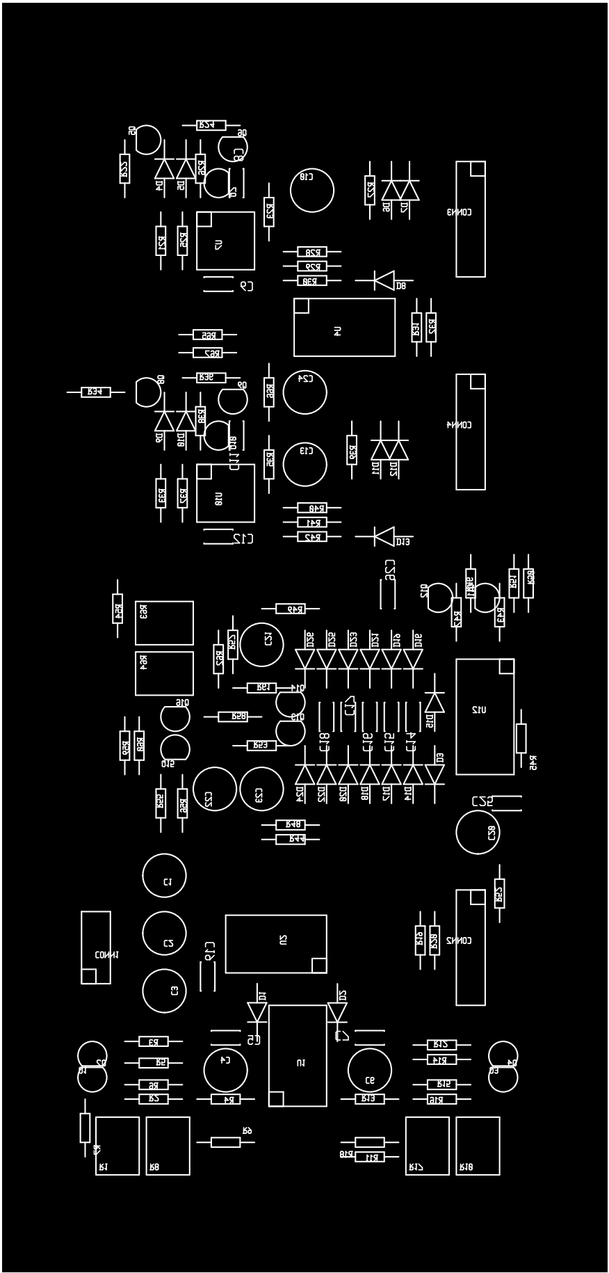
frontsilk (mirrored), scale = 1:1.080 pcb/main.pcb
