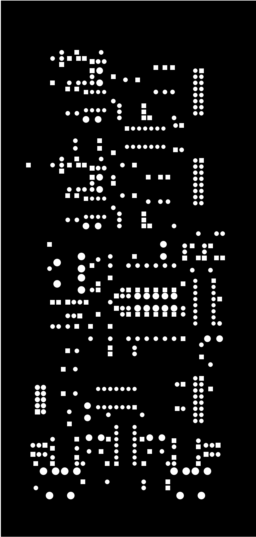
frontmask (mirrored), scale = 1:1.080 pcb/main.pcb
