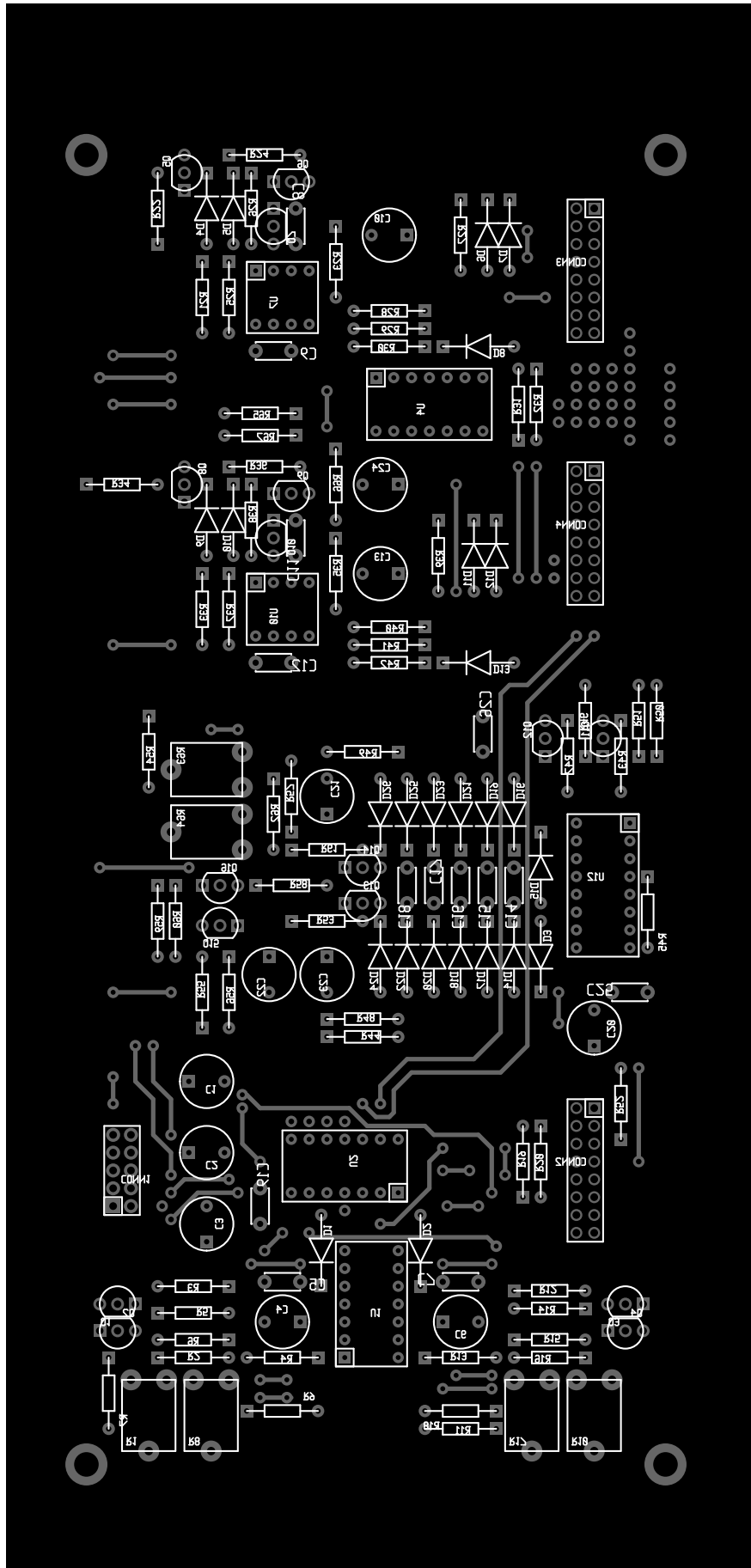
frontassembly (mirrored), scale = 1:1.080 pcb/main.pcb
